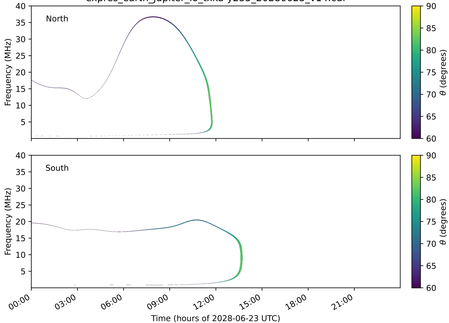
expres_earth_jupiter_io_txka-y235_20280623_v14.cdf
