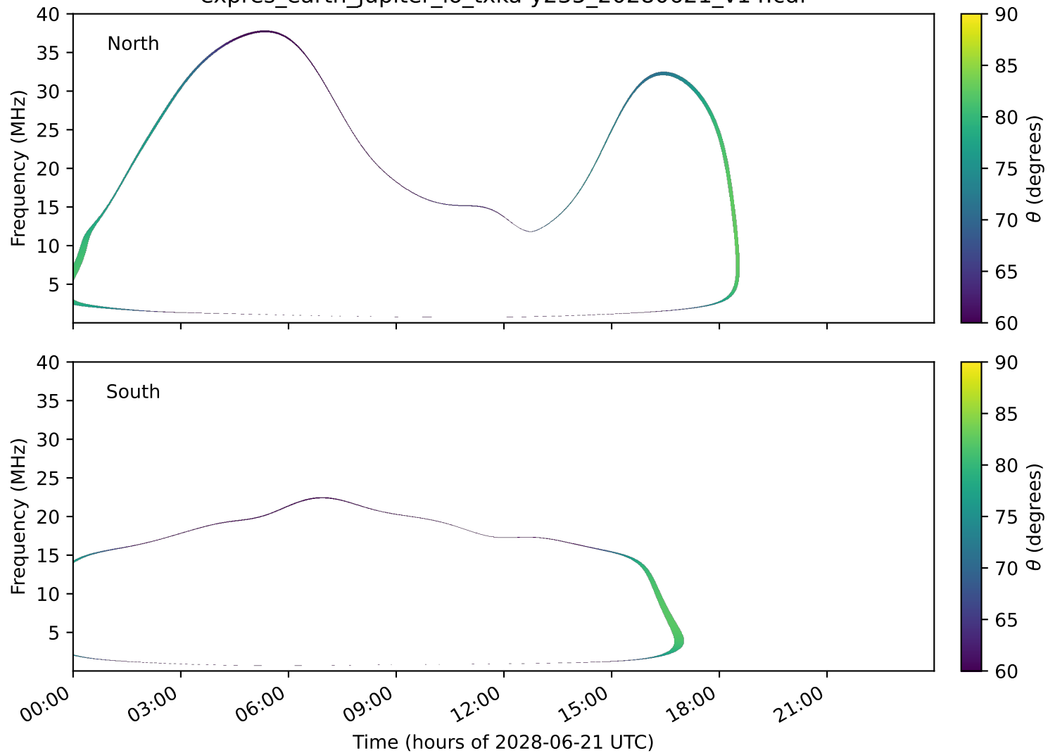
expres_earth_jupiter_io_txka-y235_20280621_v14.cdf
