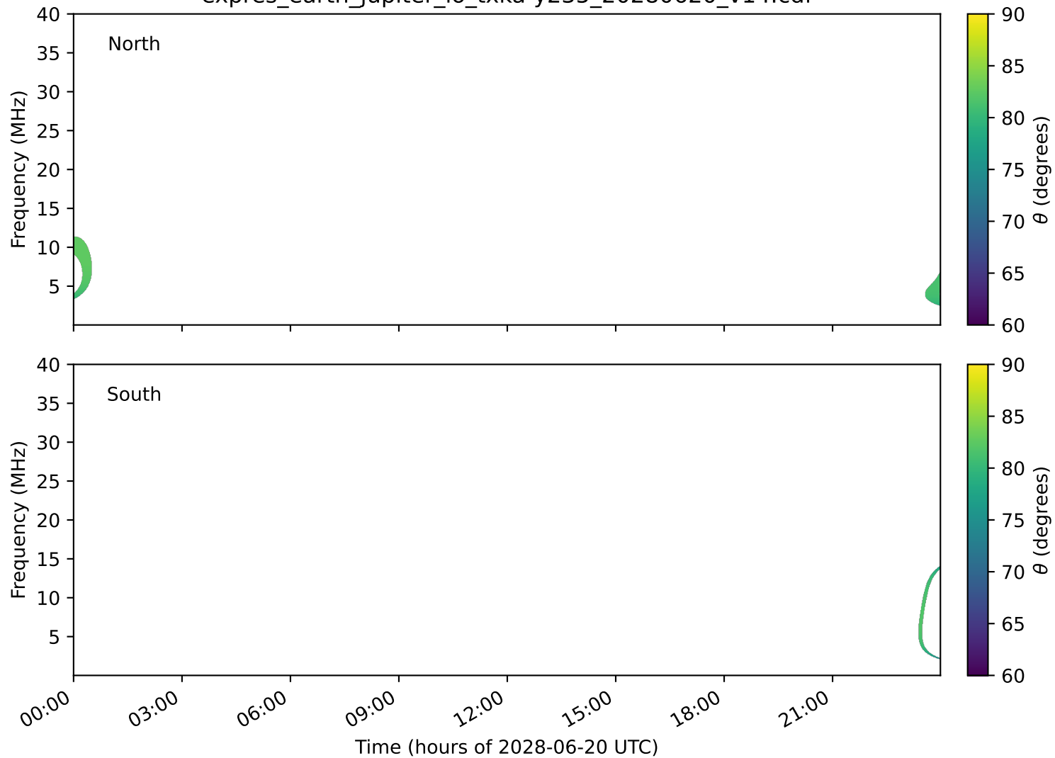
expres_earth_jupiter_io_txka-y235_20280620_v14.cdf
