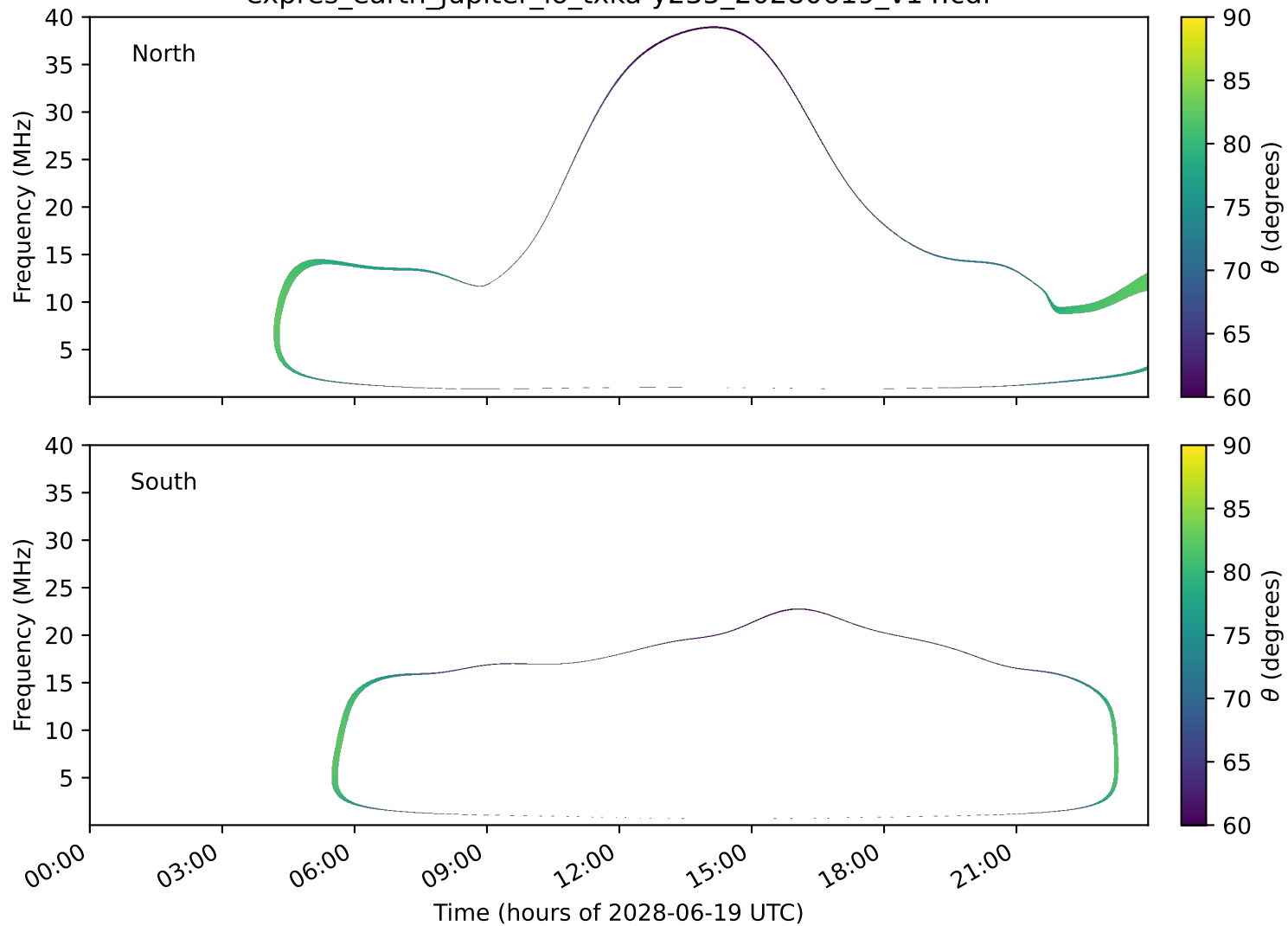
expres_earth_jupiter_io_txka-y235_20280619_v14.cdf
