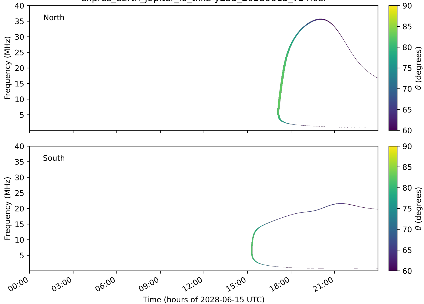
expres_earth_jupiter_io_txka-y235_20280615_v14.cdf
