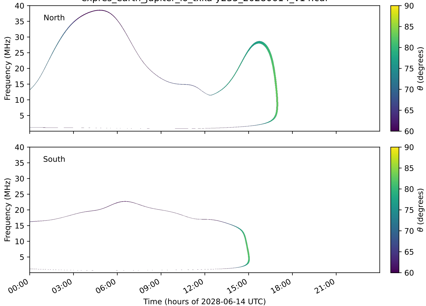
expres_earth_jupiter_io_txka-y235_20280614_v14.cdf
