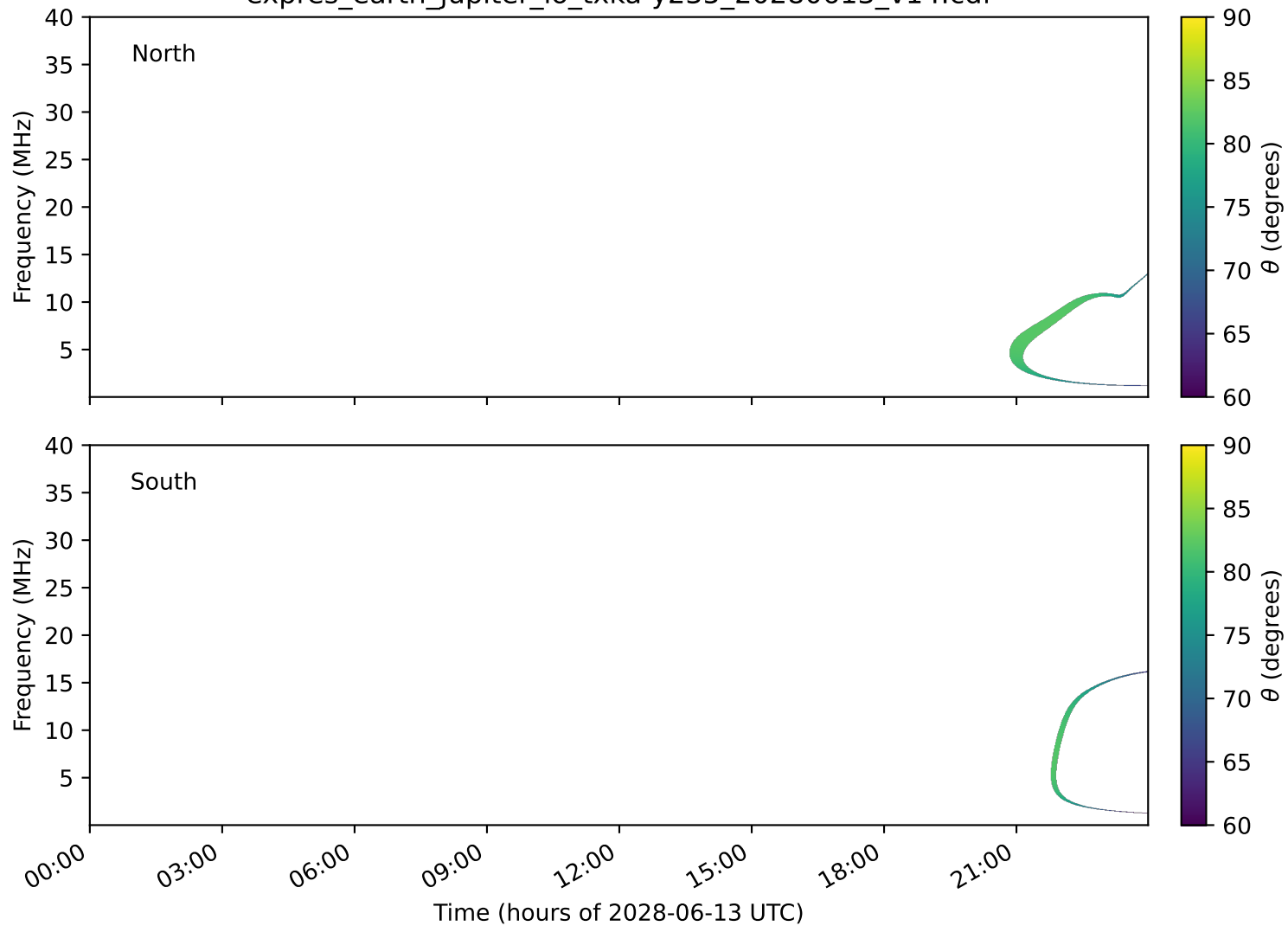
expres_earth_jupiter_io_txka-y235_20280613_v14.cdf
