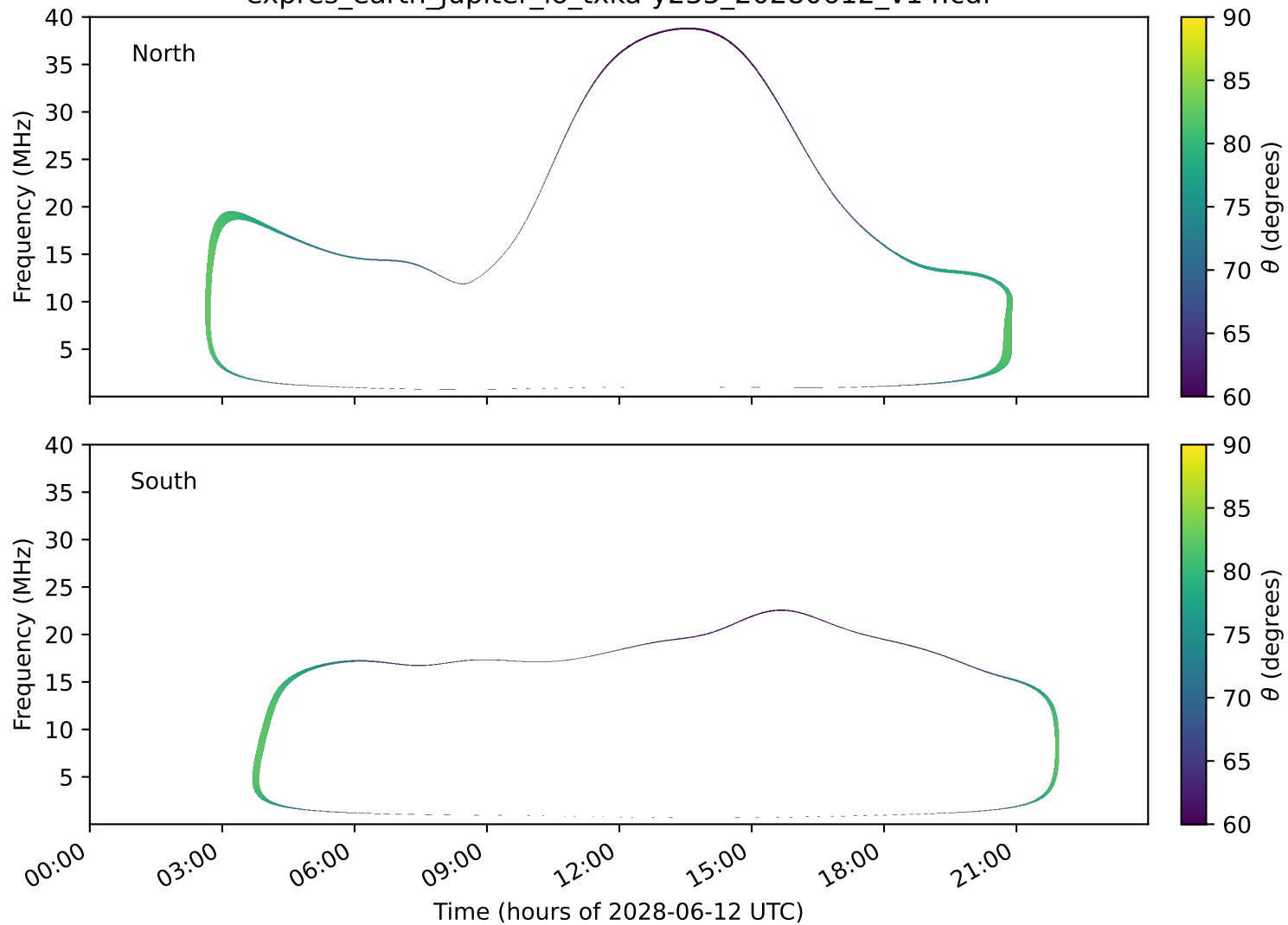
expres_earth_jupiter_io_txka-y235_20280612_v14.cdf
