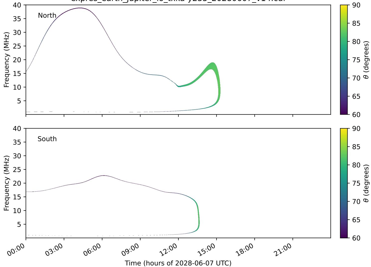
expres_earth_jupiter_io_txka-y235_20280607_v14.cdf
