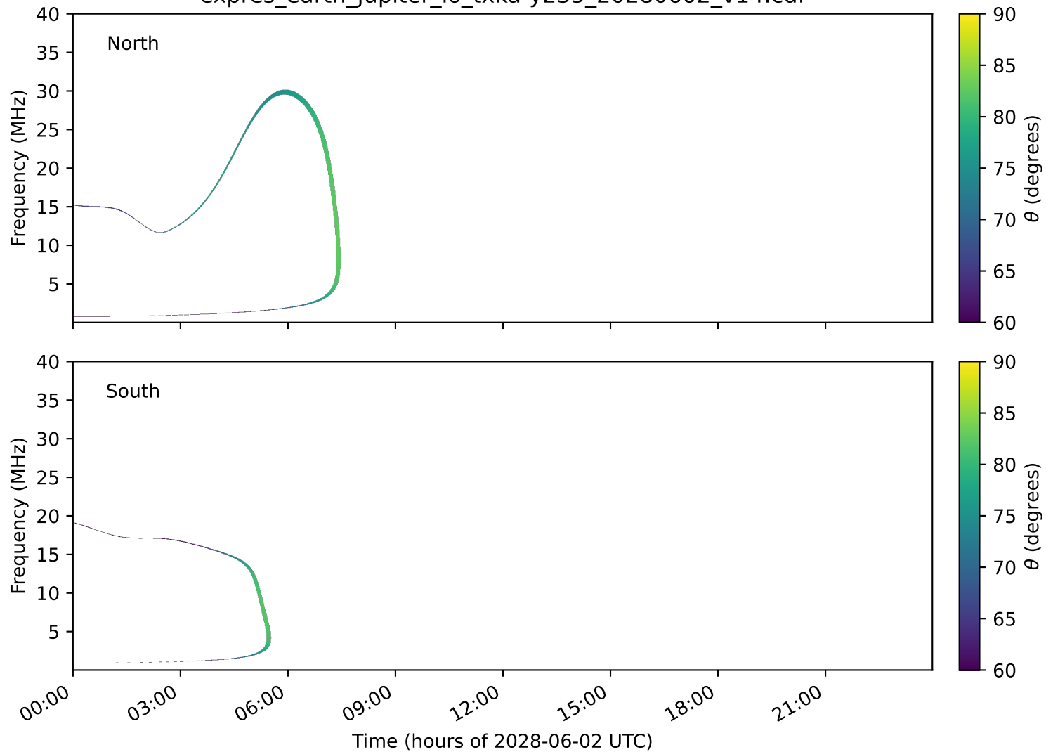
expres_earth_jupiter_io_txka-y235_20280602_v14.cdf
