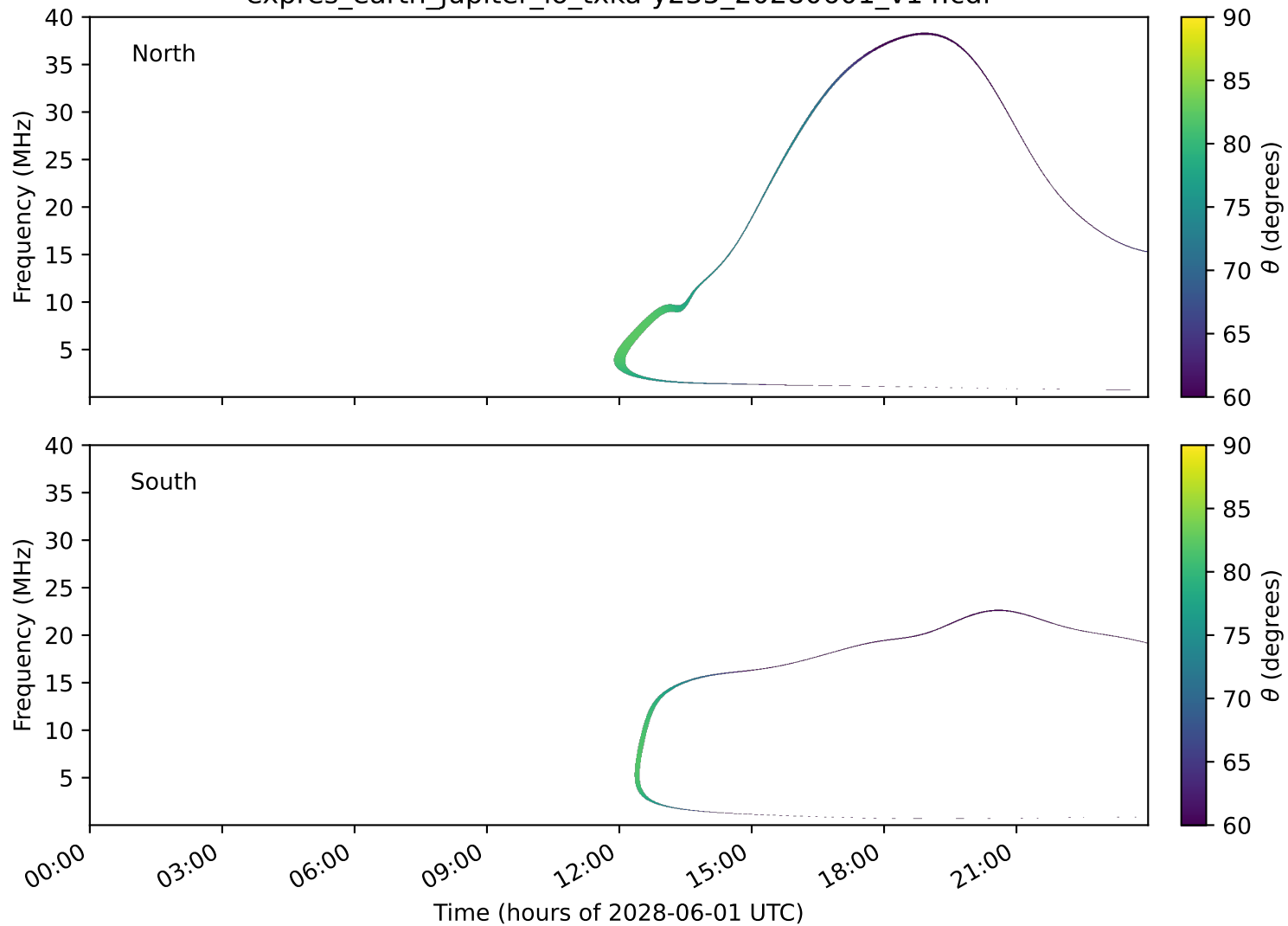
expres_earth_jupiter_io_txka-y235_20280601_v14.cdf
