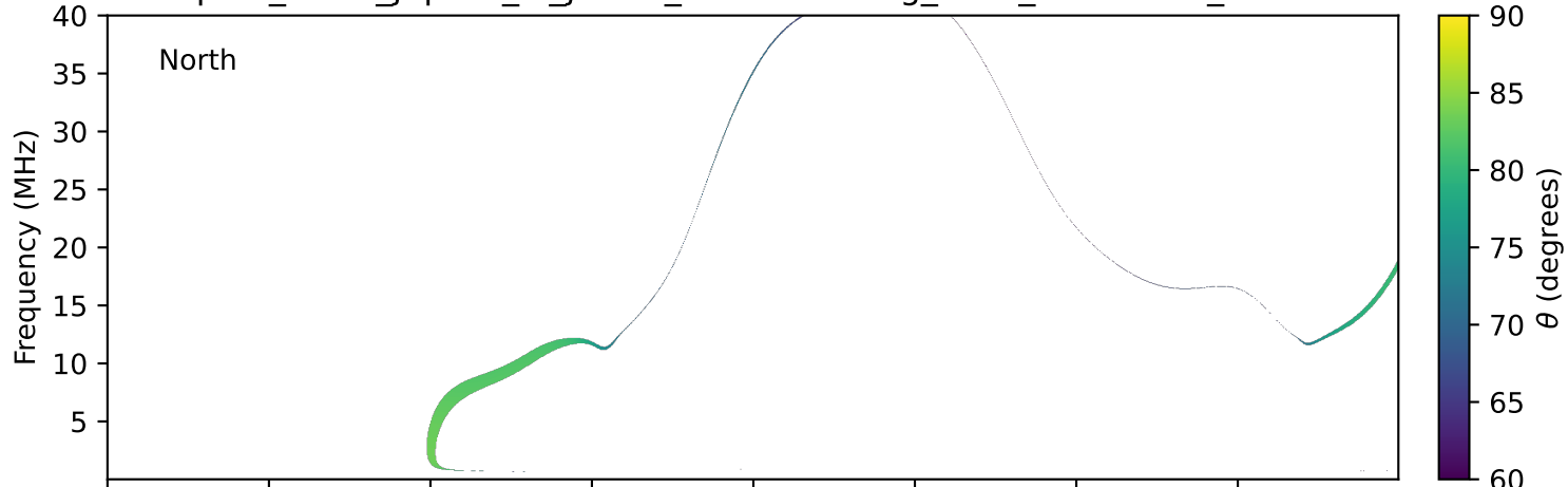
expres_earth_jupiter_io_jrm33_lossc-wid1deg_3kev_20280626_v11.cdf
