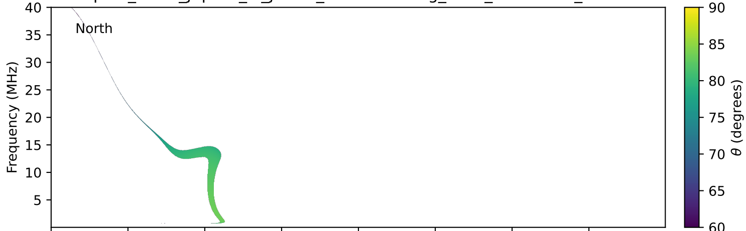
expres_earth_jupiter_io_jrm33_lossc-wid1deg_3kev_20280625_v11.cdf
