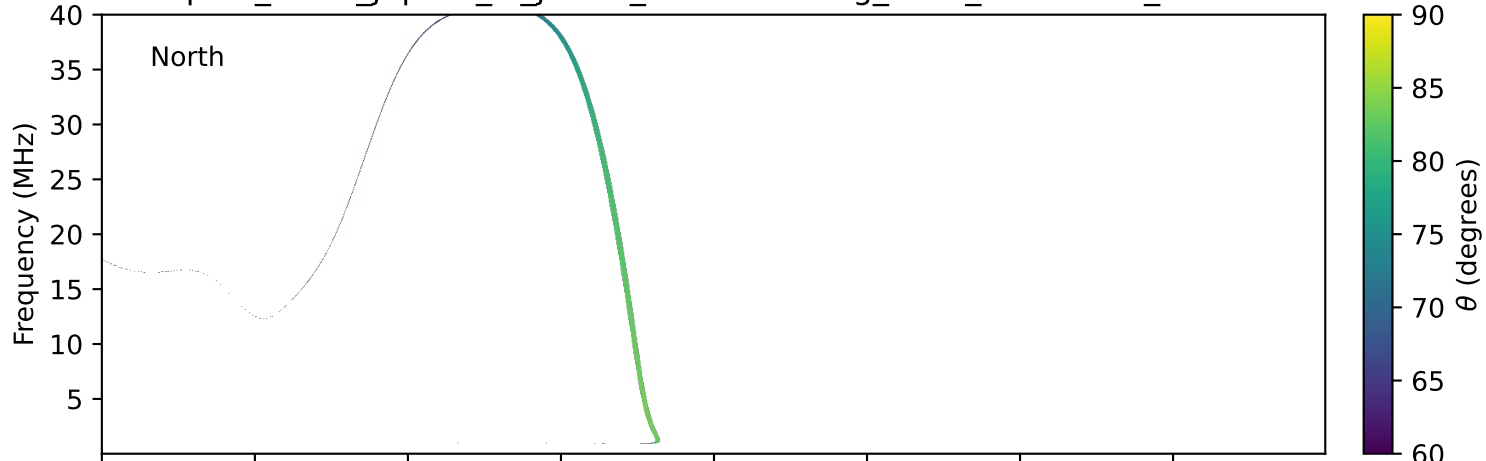
expres_earth_jupiter_io_jrm33_lossc-wid1deg_3kev_20280616_v11.cdf
