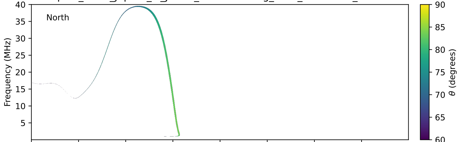
expres_earth_jupiter_io_jrm33_lossc-wid1deg_3kev_20280609_v11.cdf
