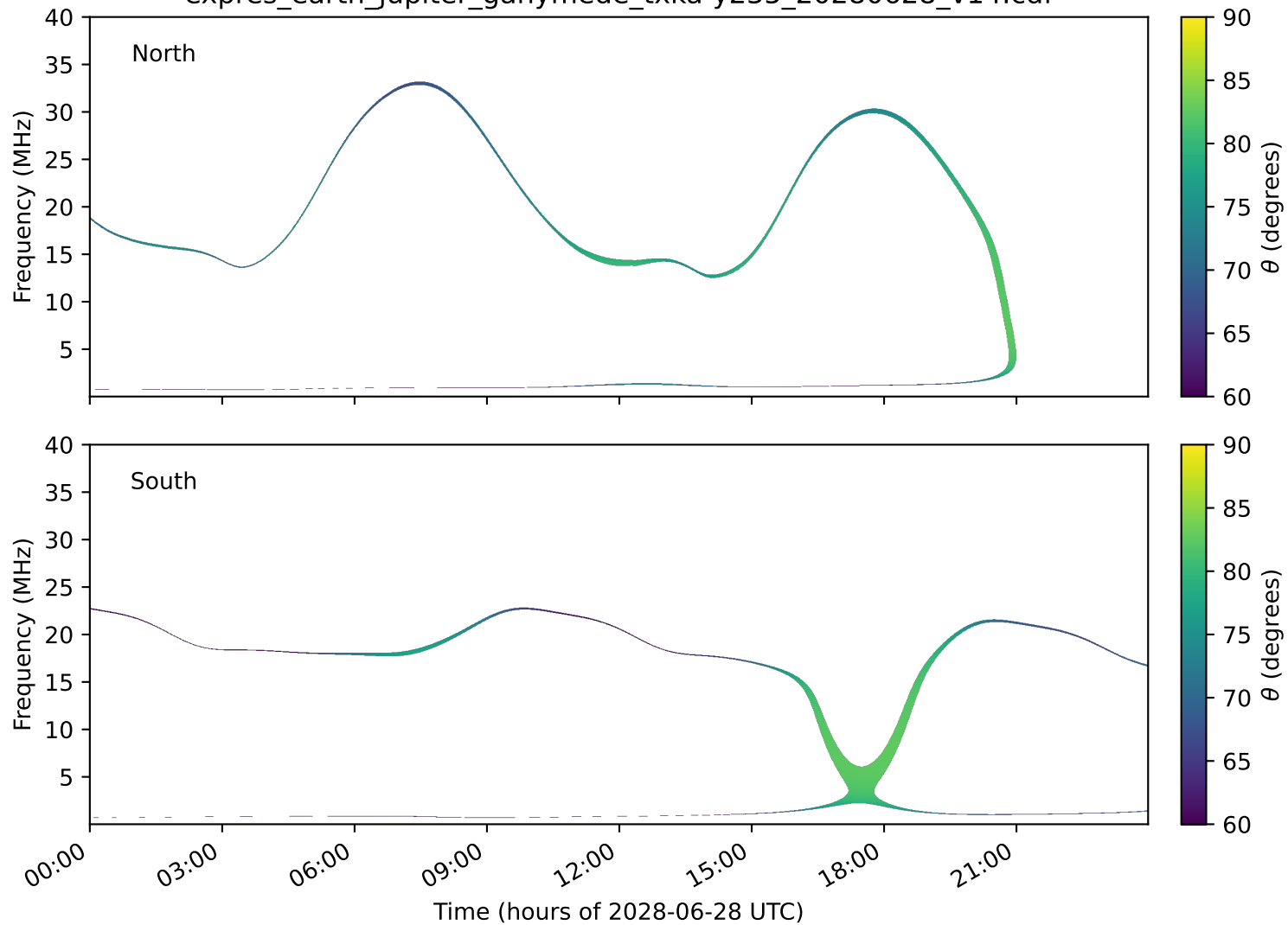
expres_earth_jupiter_ganymede_txka-y235_20280628_v14.cdf
