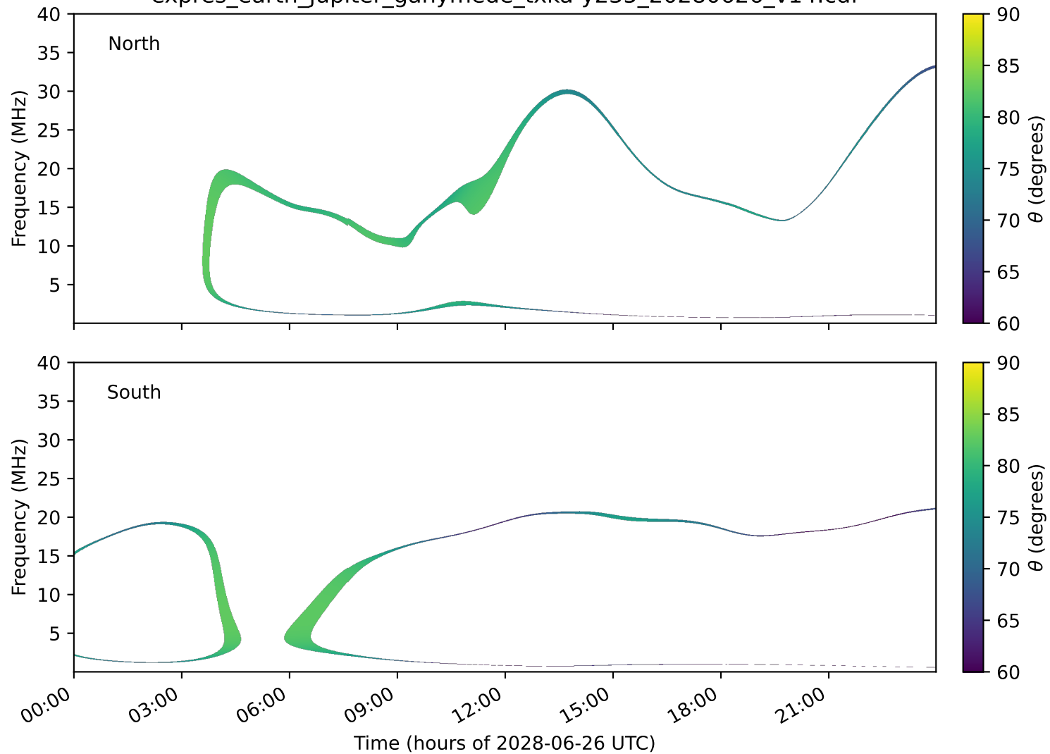
expres_earth_jupiter_ganymede_txka-y235_20280626_v14.cdf
