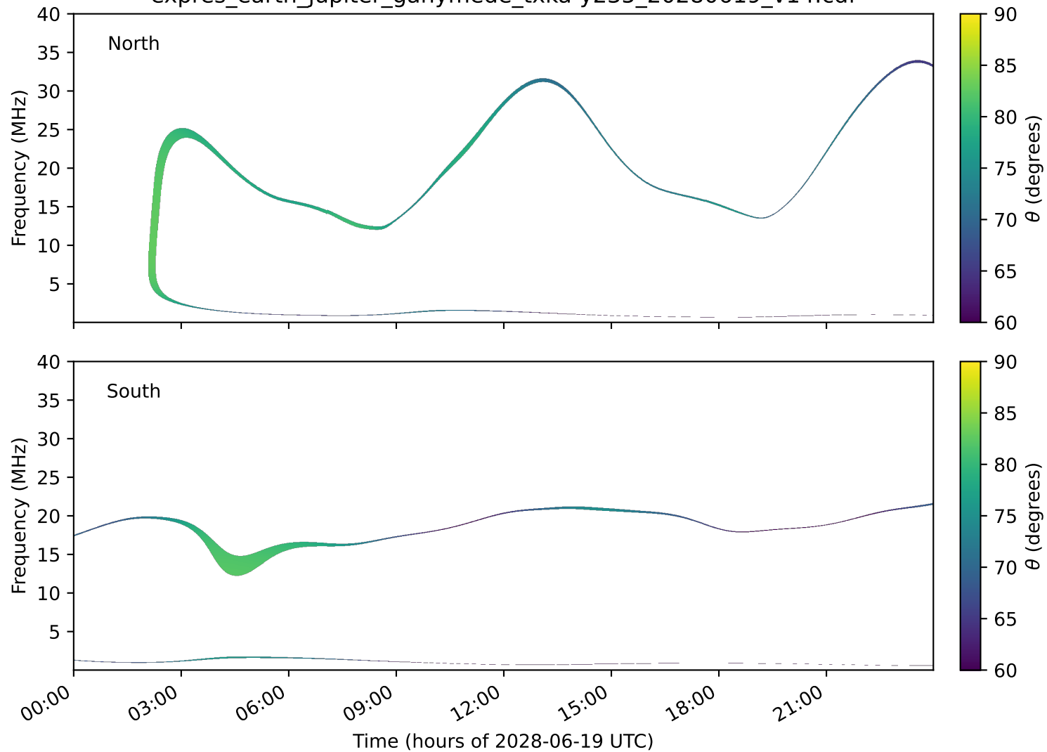
expres_earth_jupiter_ganymede_txka-y235_20280619_v14.cdf
