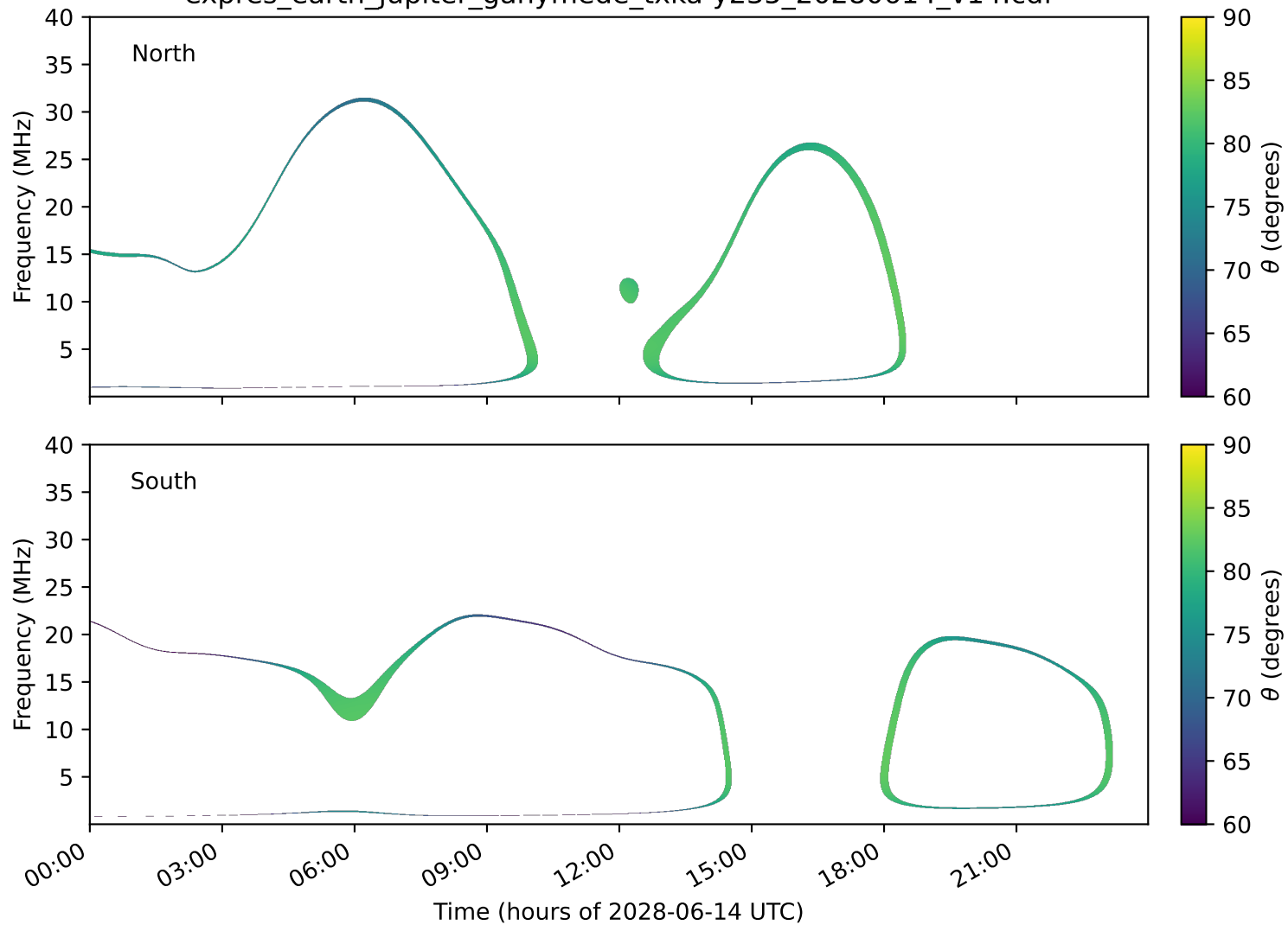
expres_earth_jupiter_ganymede_txka-y235_20280614_v14.cdf
