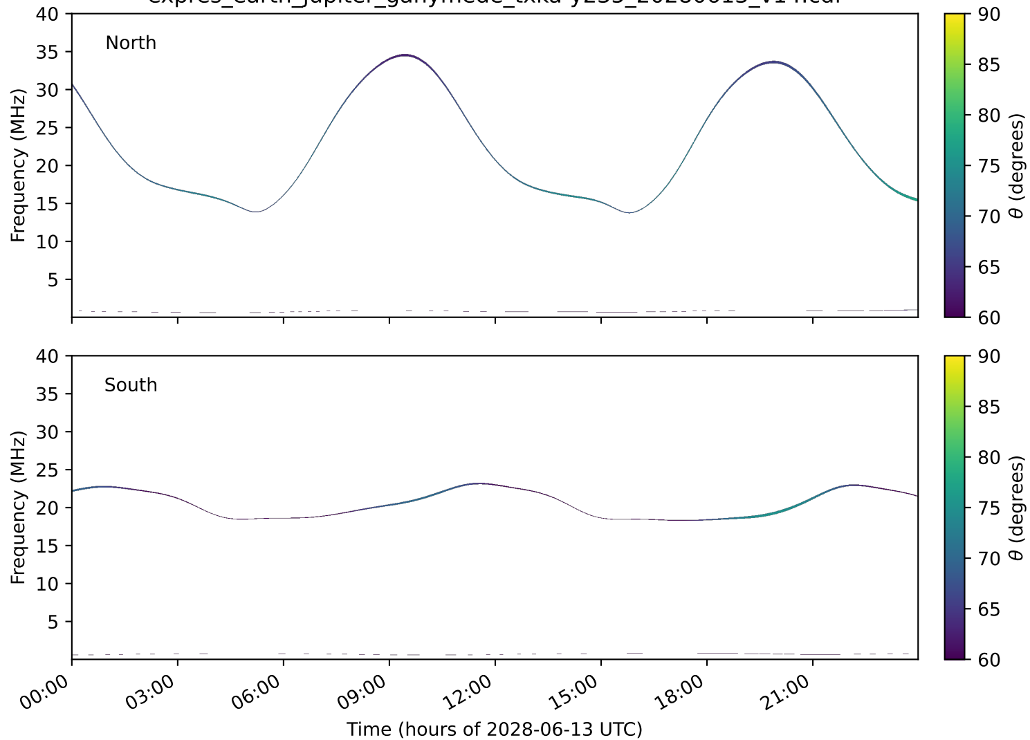
expres_earth_jupiter_ganymede_txka-y235_20280613_v14.cdf
