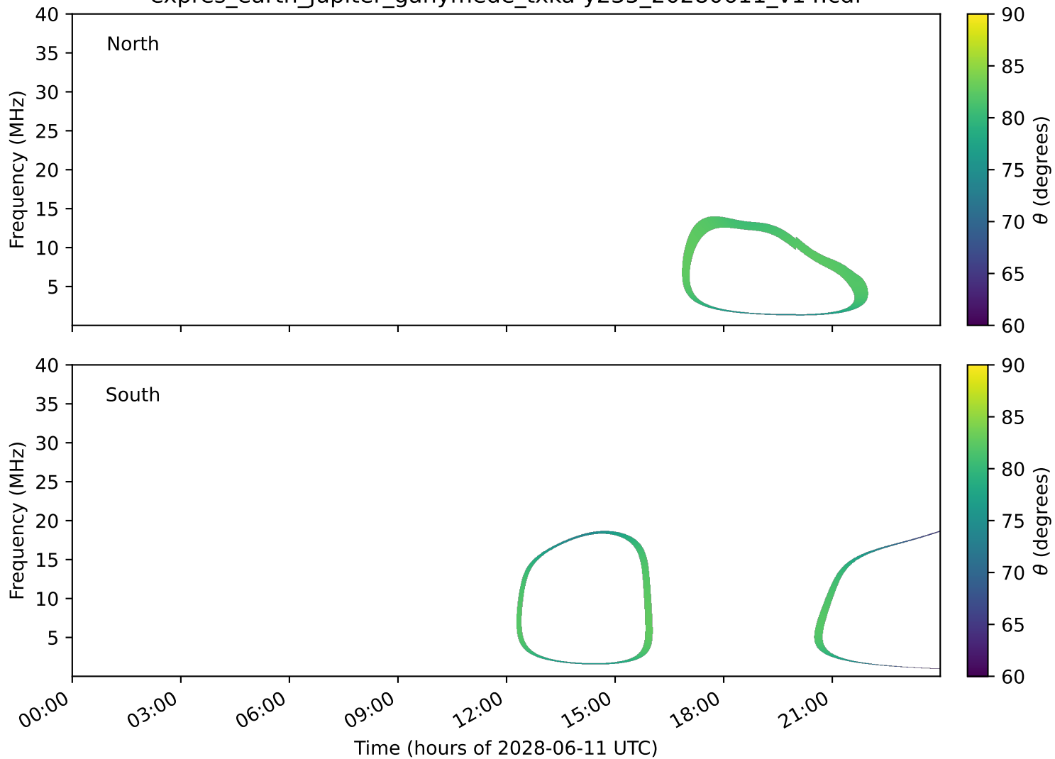
expres_earth_jupiter_ganymede_txka-y235_20280611_v14.cdf
