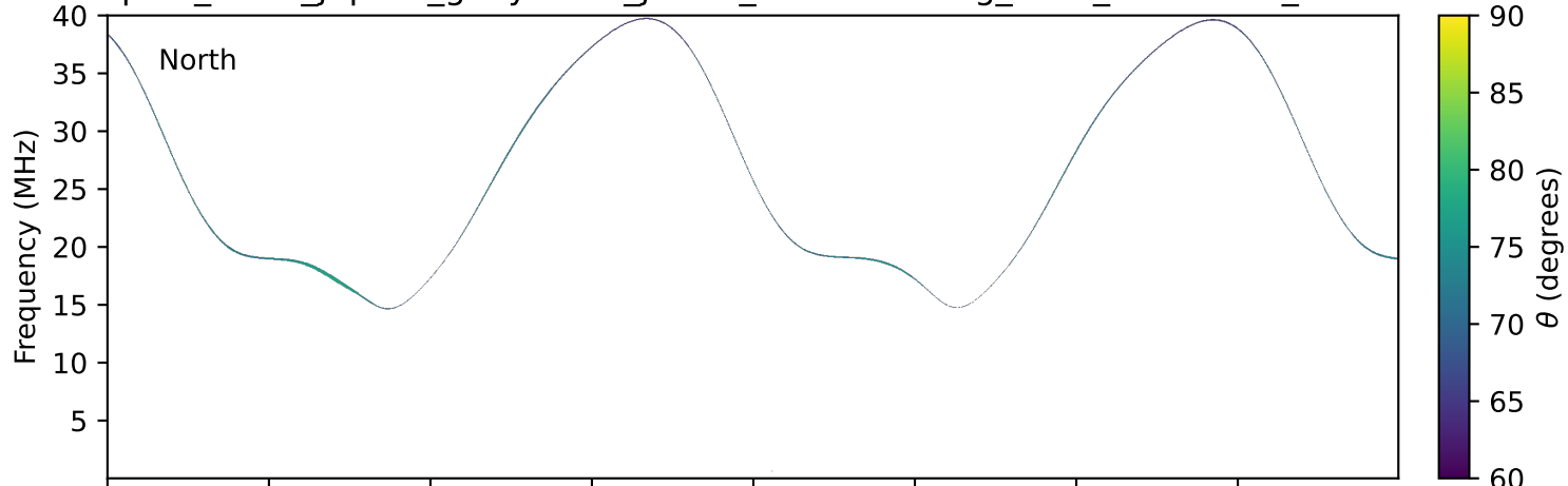
expres_earth_jupiter_ganymede_jrm33_lossc-wid1deg_3kev_20280620_v11.cdf
