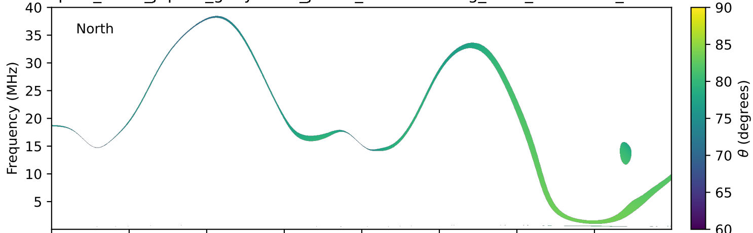
expres_earth_jupiter_ganymede_jrm33_lossc-wid1deg_3kev_20280614_v11.cdf
