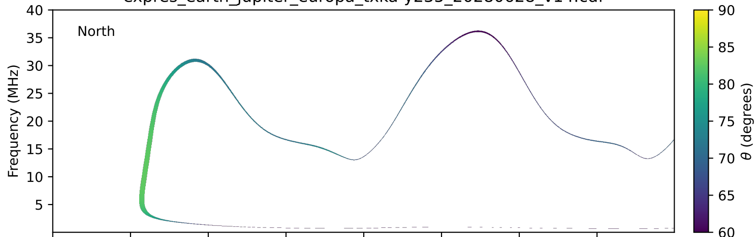
expres_earth_jupiter_europa_txka-y235_20280628_v14.cdf
