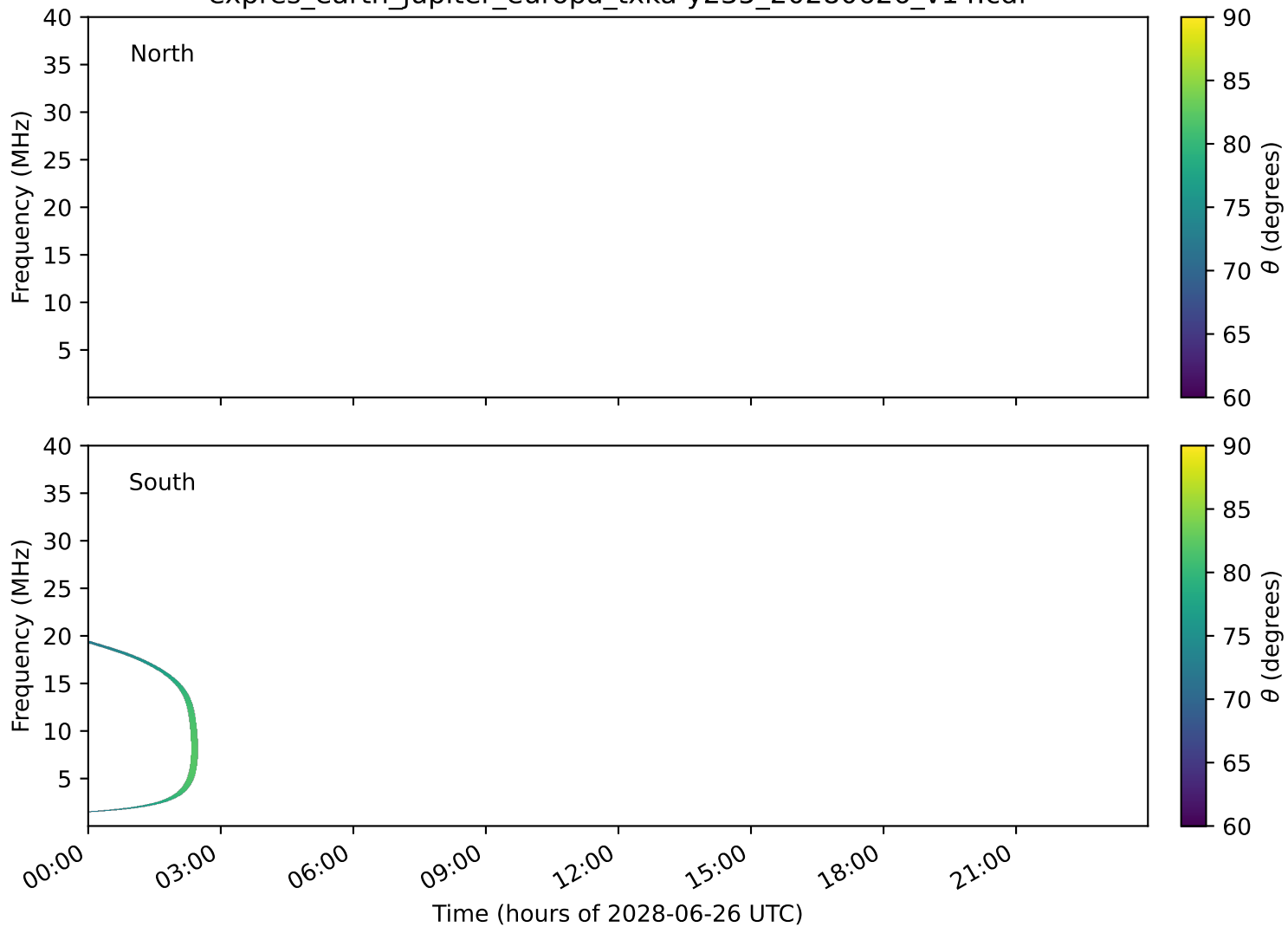
expres_earth_jupiter_europa_txka-y235_20280626_v14.cdf
