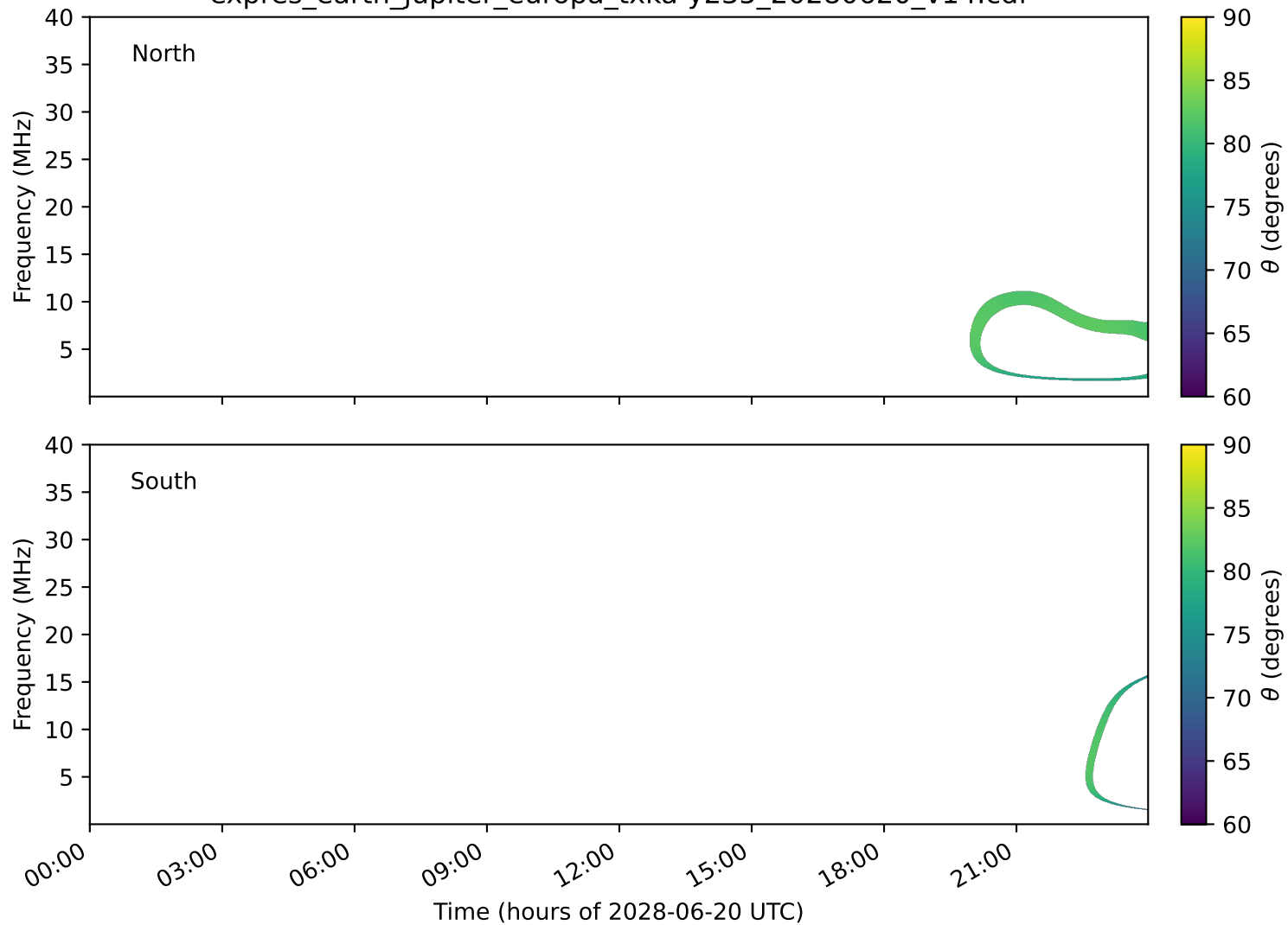
expres_earth_jupiter_europa_txka-y235_20280620_v14.cdf
