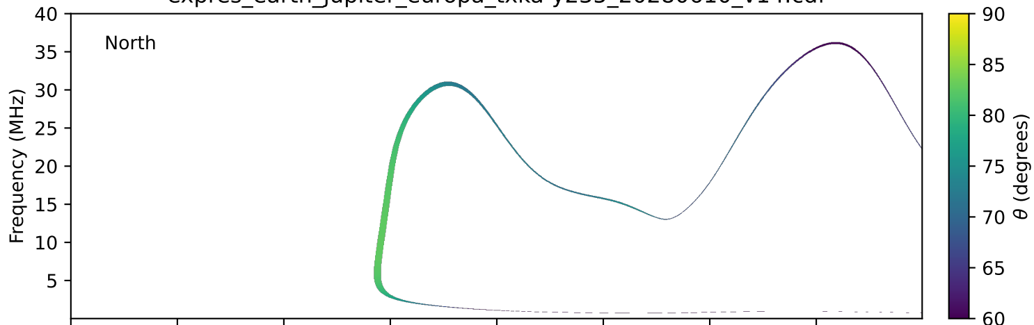
expres_earth_jupiter_europa_txka-y235_20280610_v14.cdf
