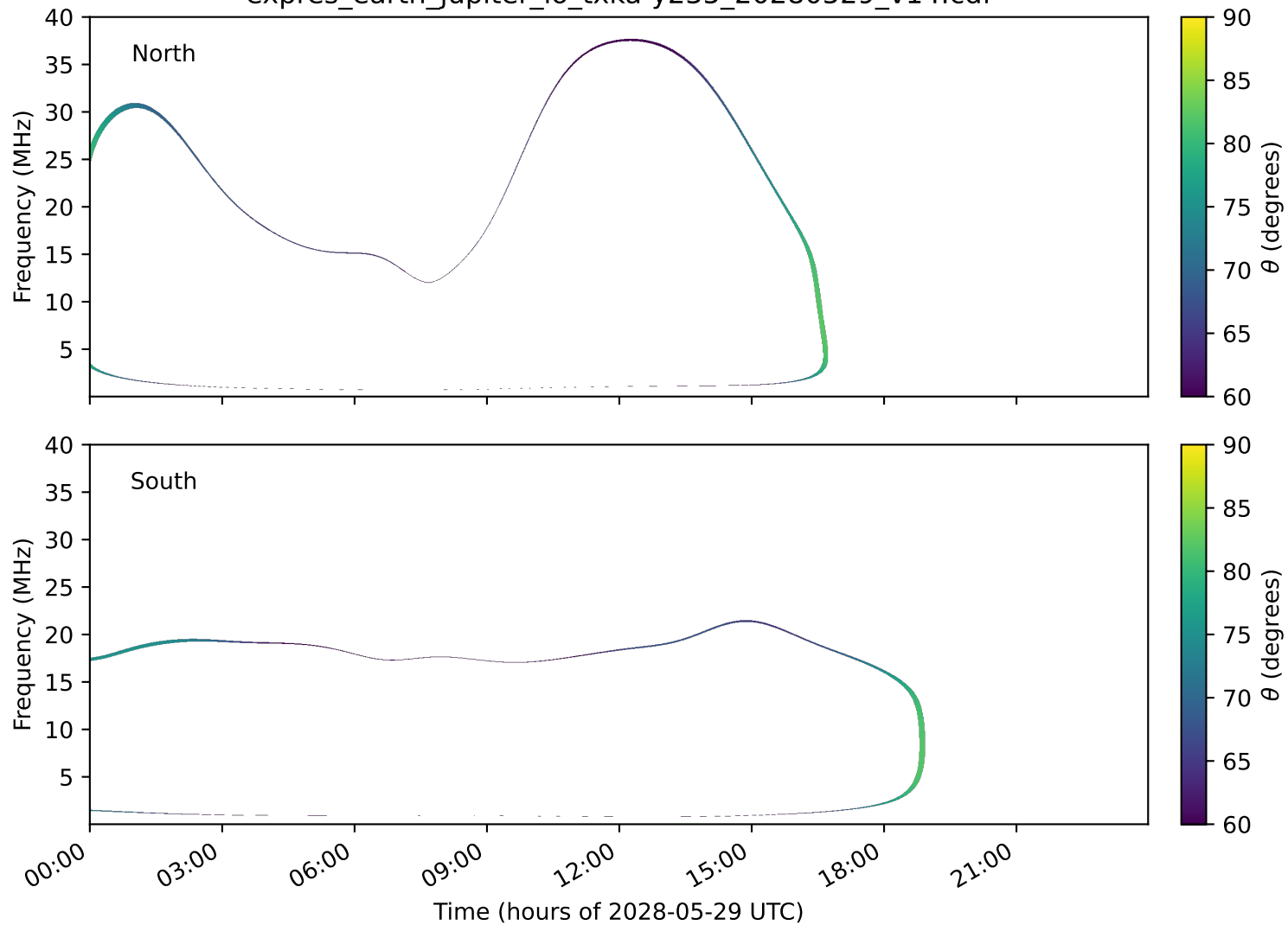
expres_earth_jupiter_io_txka-y235_20280529_v14.cdf
