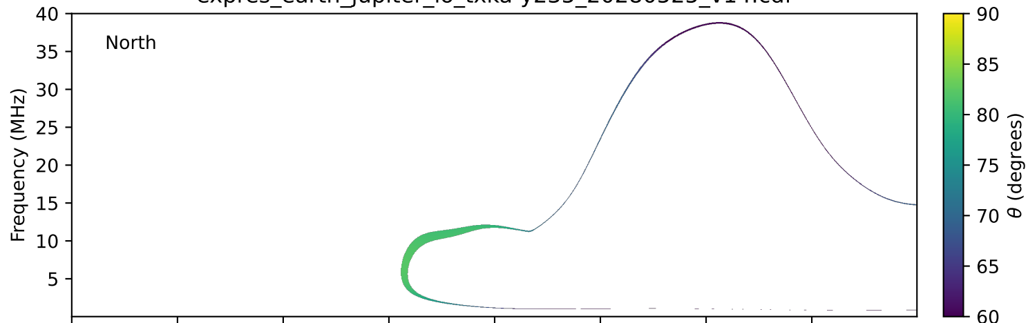
expres_earth_jupiter_io_txka-y235_20280525_v14.cdf
