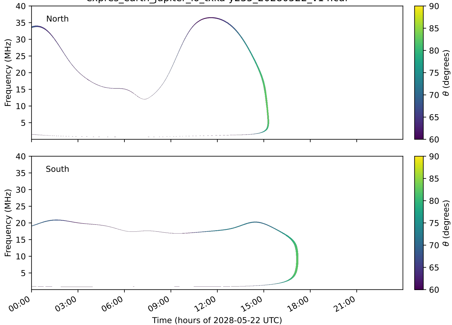
expres_earth_jupiter_io_txka-y235_20280522_v14.cdf
