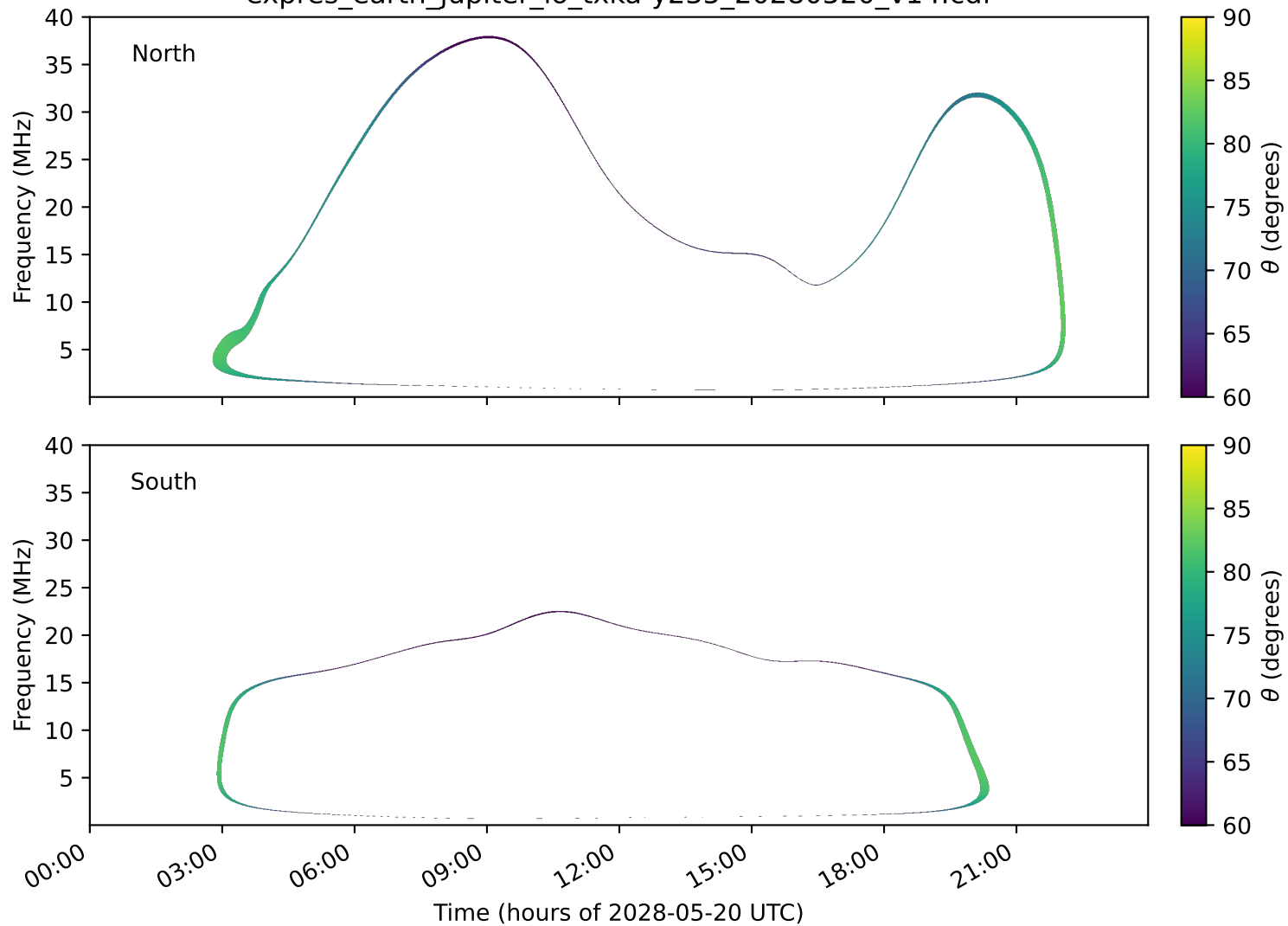
expres_earth_jupiter_io_txka-y235_20280520_v14.cdf
