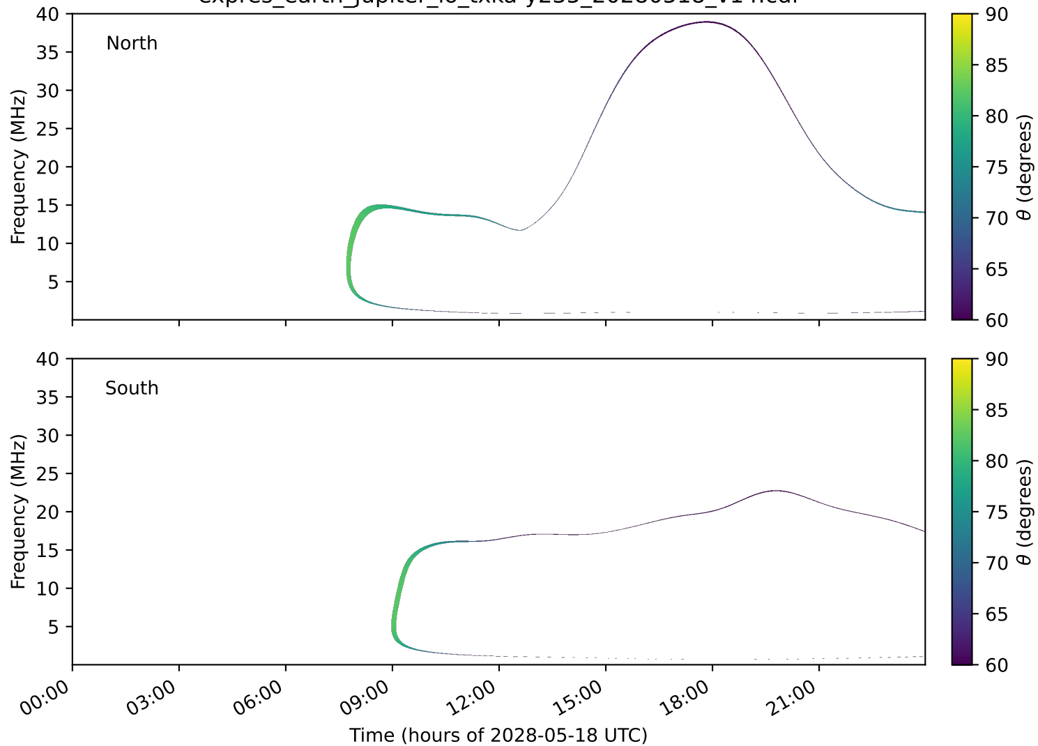
expres_earth_jupiter_io_txka-y235_20280518_v14.cdf
