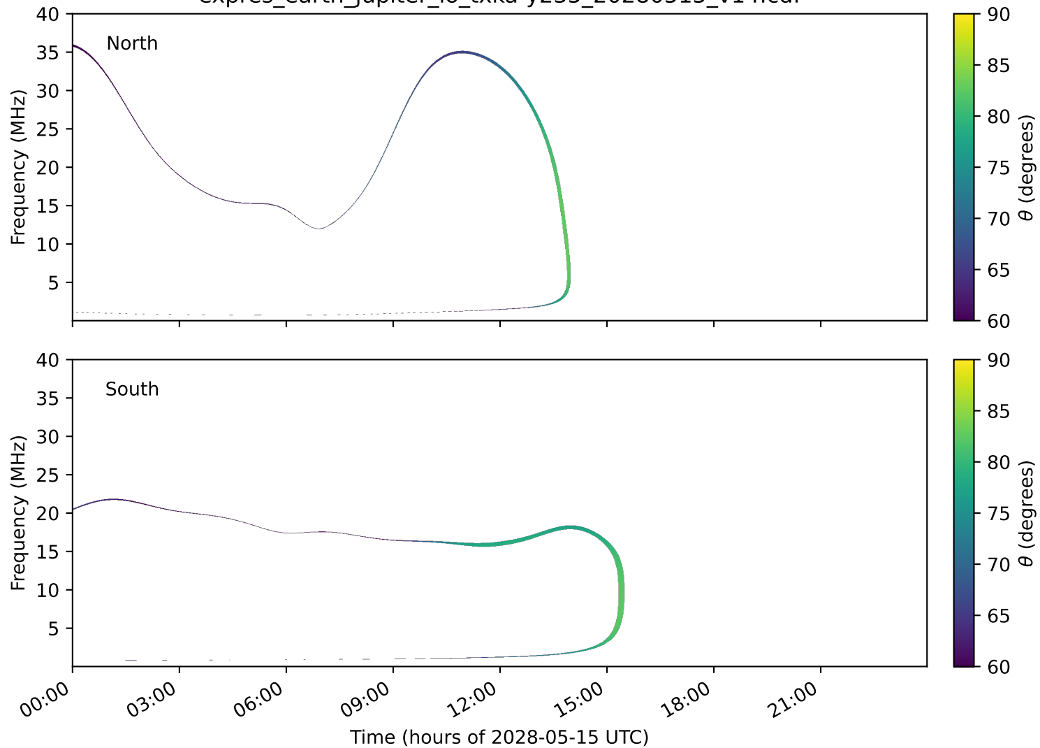
expres_earth_jupiter_io_txka-y235_20280515_v14.cdf
