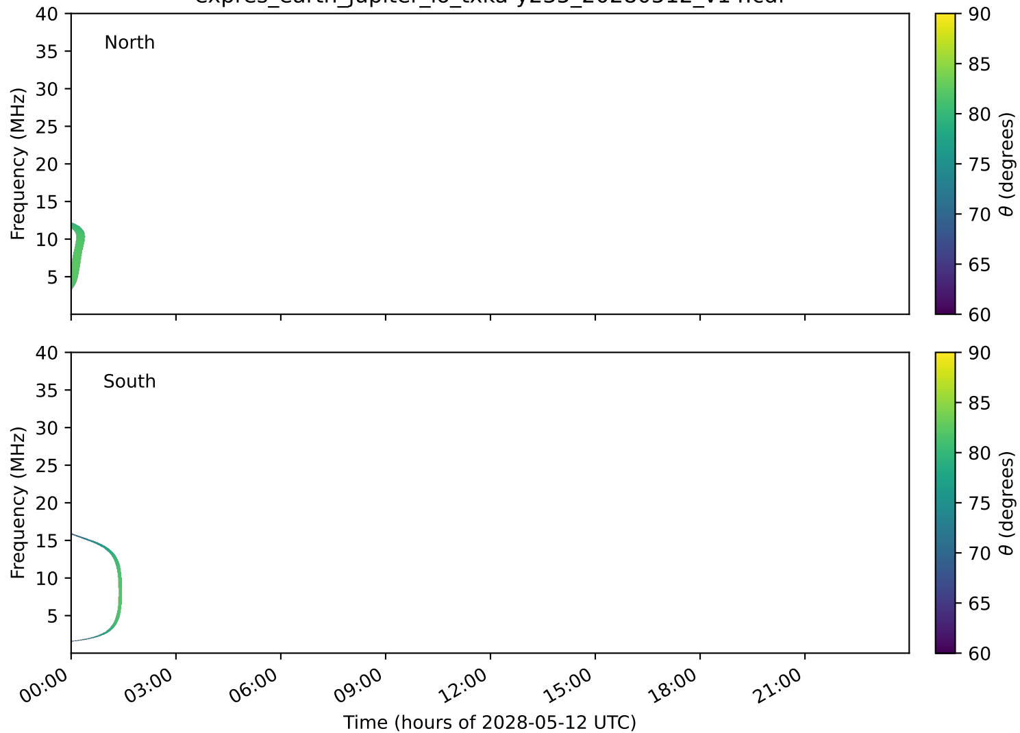
expres_earth_jupiter_io_txka-y235_20280512_v14.cdf
