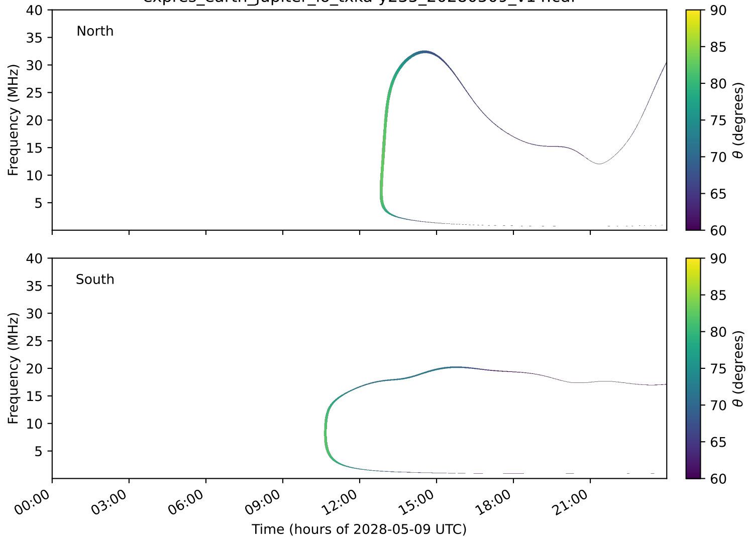
expres_earth_jupiter_io_txka-y235_20280509_v14.cdf
