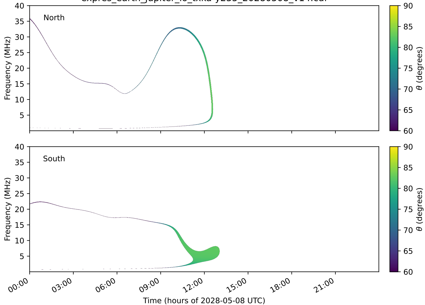
expres_earth_jupiter_io_txka-y235_20280508_v14.cdf
