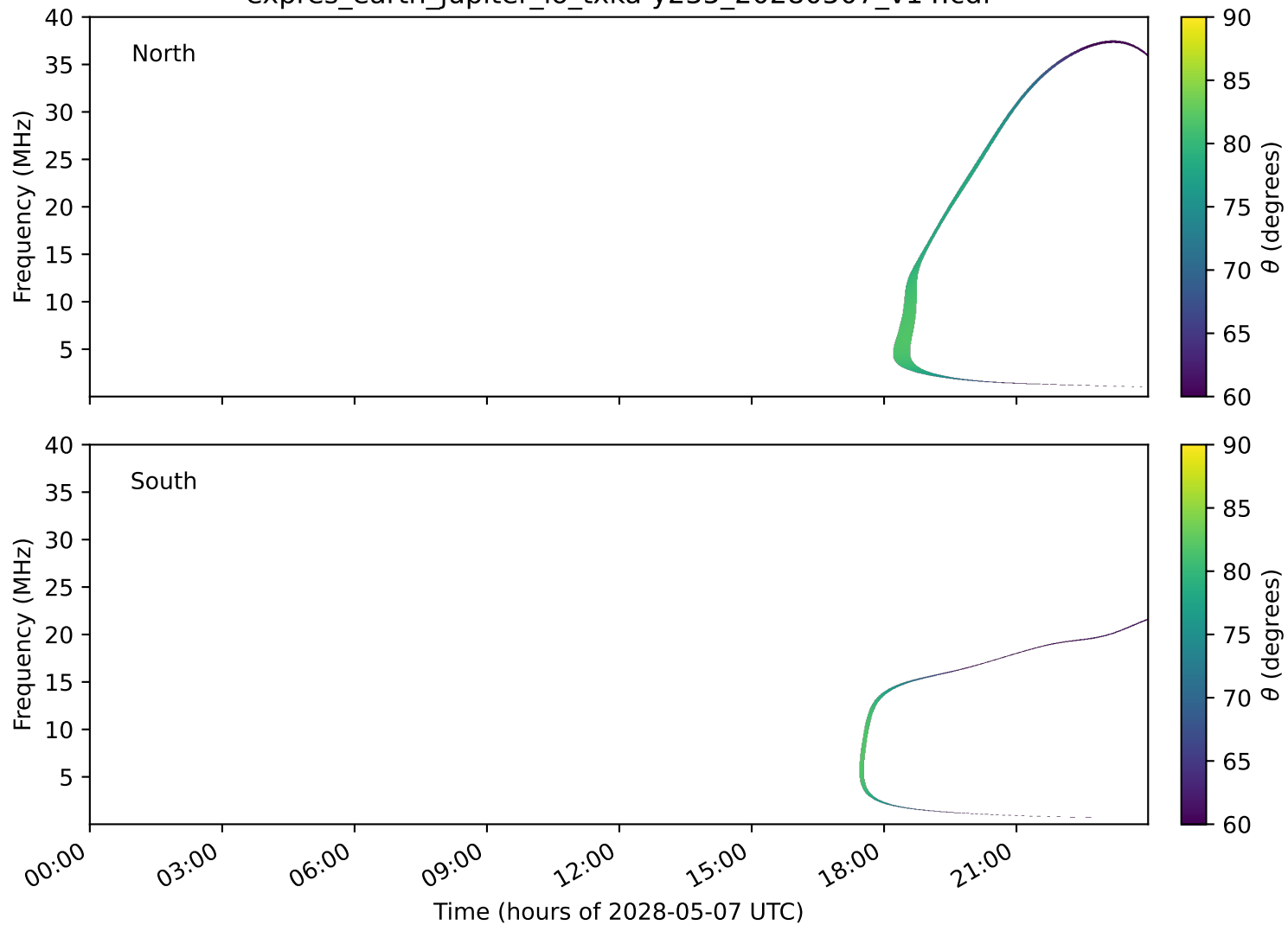
expres_earth_jupiter_io_txka-y235_20280507_v14.cdf
