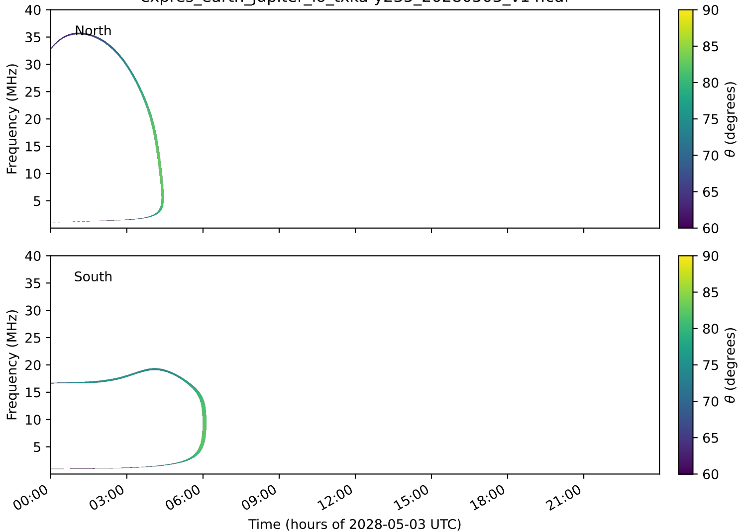
expres_earth_jupiter_io_txka-y235_20280503_v14.cdf
