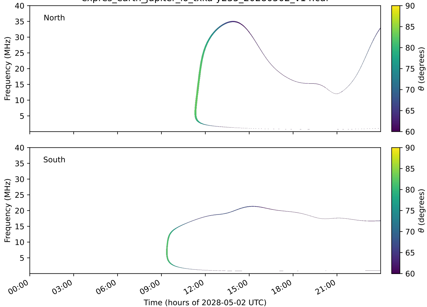
expres_earth_jupiter_io_txka-y235_20280502_v14.cdf
