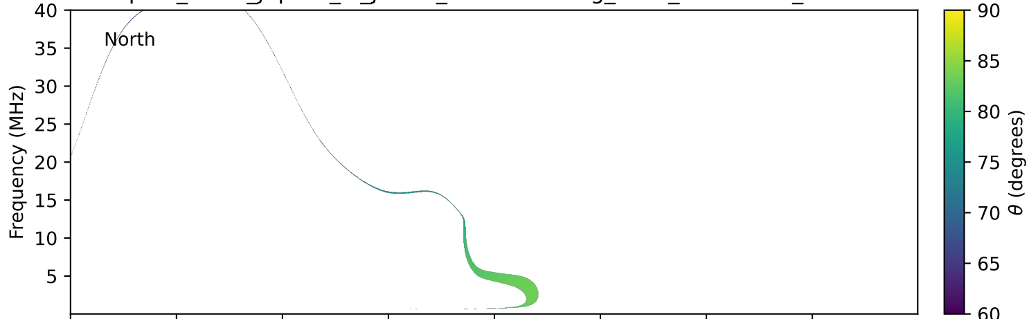
expres_earth_jupiter_io_jrm33_lossc-wid1deg_3kev_20280531_v11.cdf
