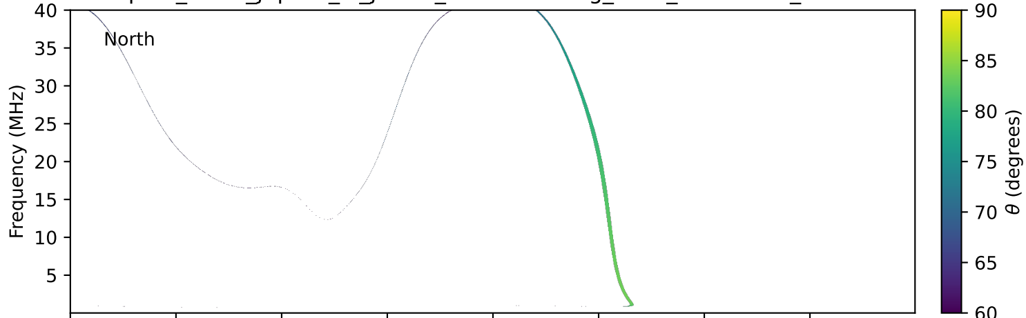
expres_earth_jupiter_io_jrm33_lossc-wid1deg_3kev_20280522_v11.cdf
