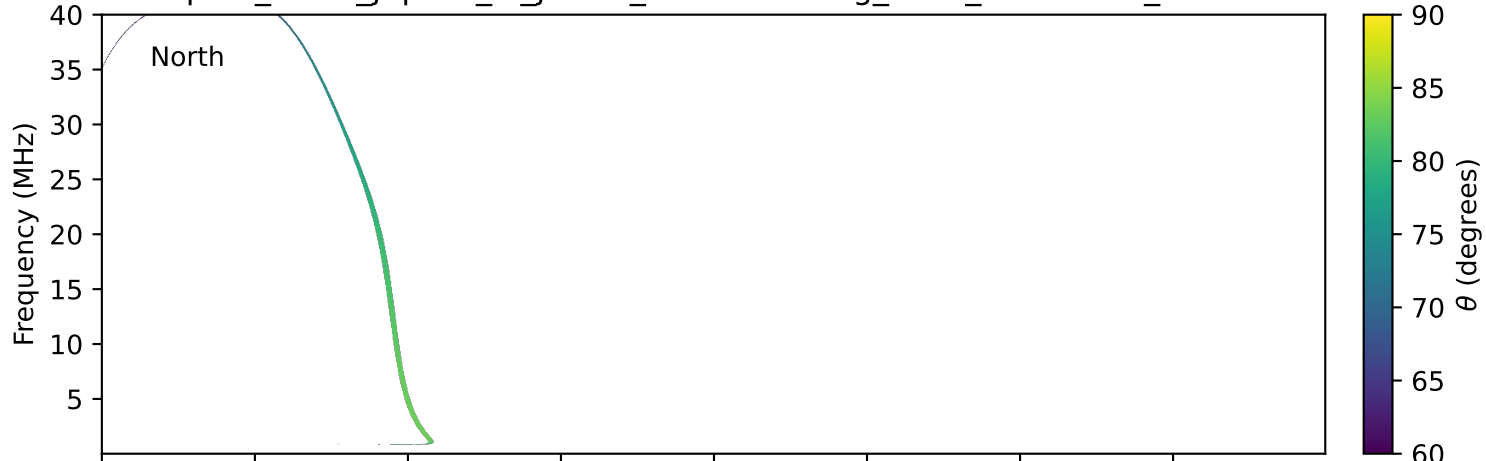
expres_earth_jupiter_io_jrm33_lossc-wid1deg_3kev_20280510_v11.cdf
