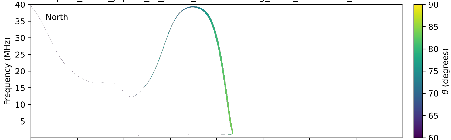
expres_earth_jupiter_io_jrm33_lossc-wid1deg_3kev_20280508_v11.cdf
