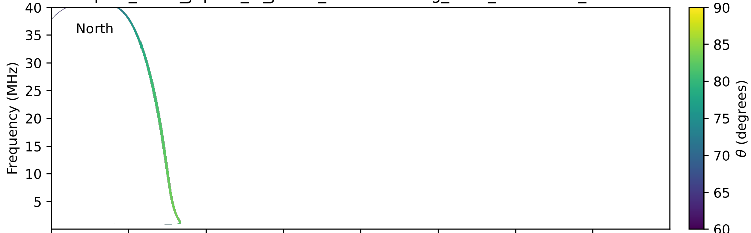
expres_earth_jupiter_io_jrm33_lossc-wid1deg_3kev_20280503_v11.cdf
