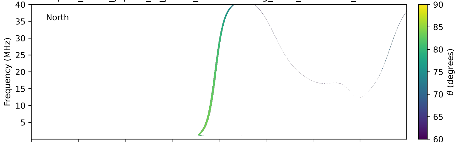
expres_earth_jupiter_io_jrm33_lossc-wid1deg_3kev_20280502_v11.cdf
