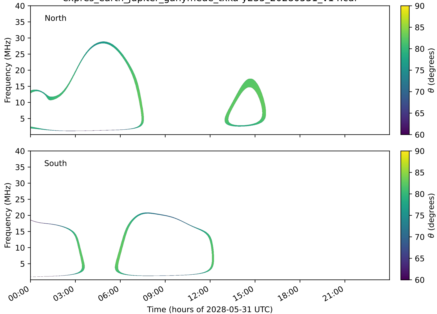
expres_earth_jupiter_ganymede_txka-y235_20280531_v14.cdf
