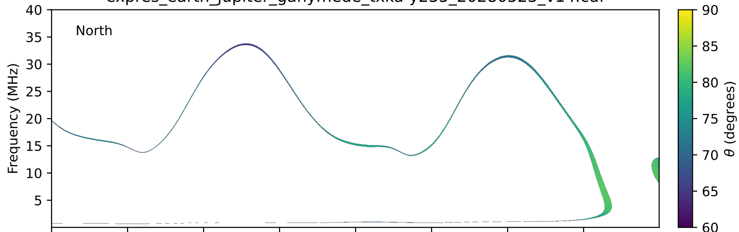
expres_earth_jupiter_ganymede_txka-y235_20280523_v14.cdf
