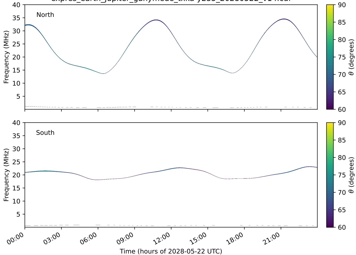
expres_earth_jupiter_ganymede_txka-y235_20280522_v14.cdf
