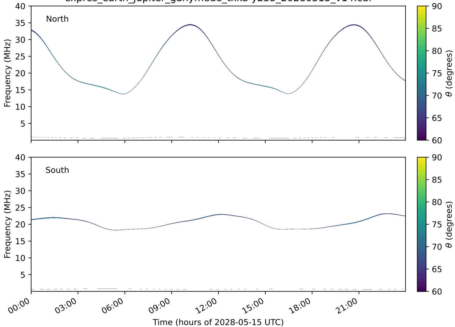
expres_earth_jupiter_ganymede_txka-y235_20280515_v14.cdf
