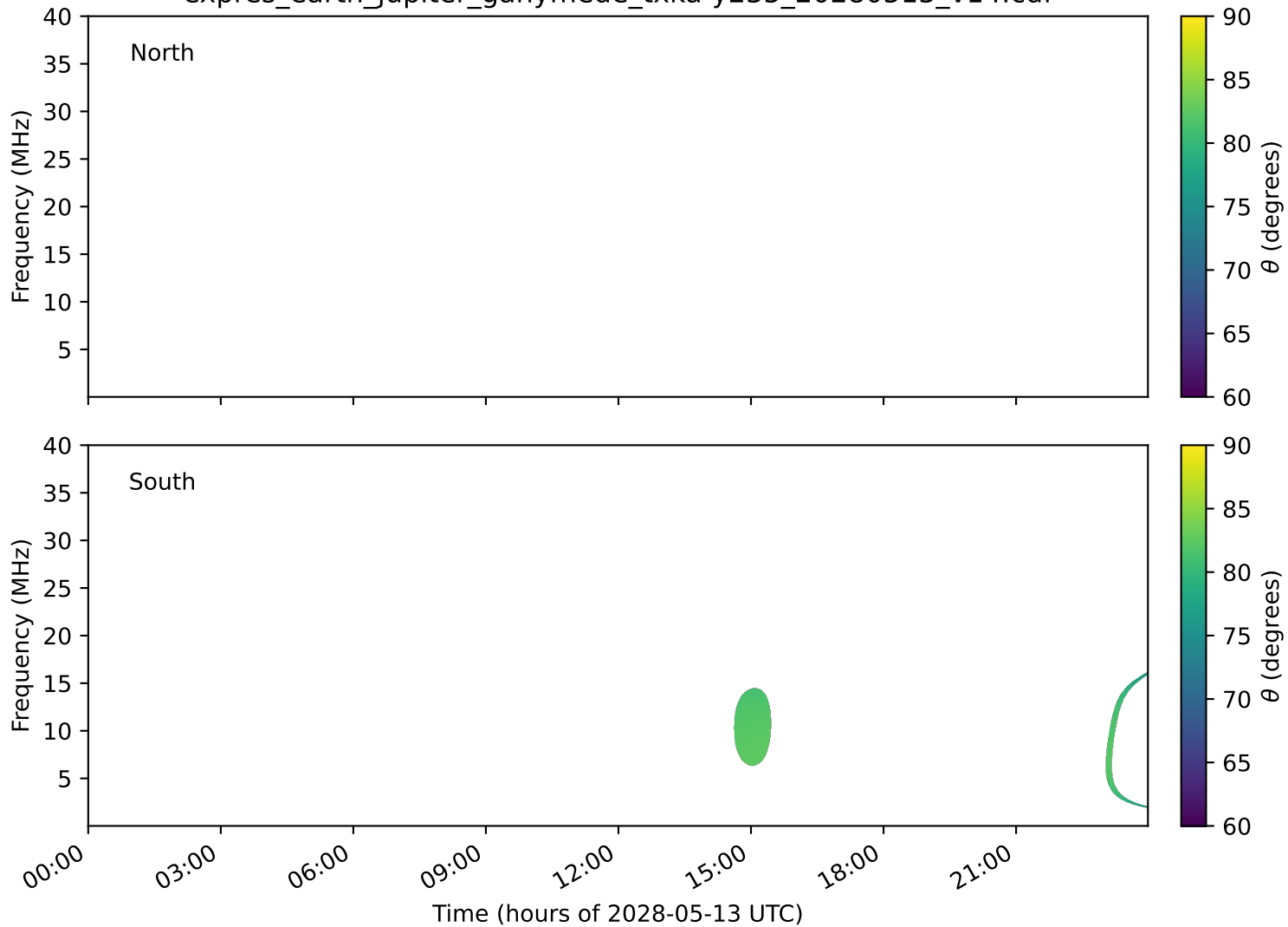
expres_earth_jupiter_ganymede_txka-y235_20280513_v14.cdf
